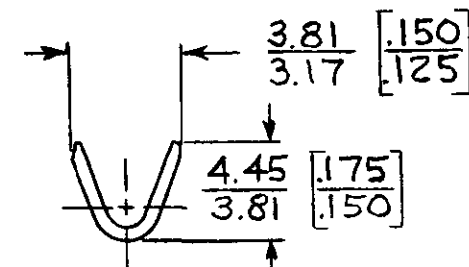
SECT. A-A
